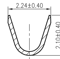
SECTION C-C SCALE 2:1
